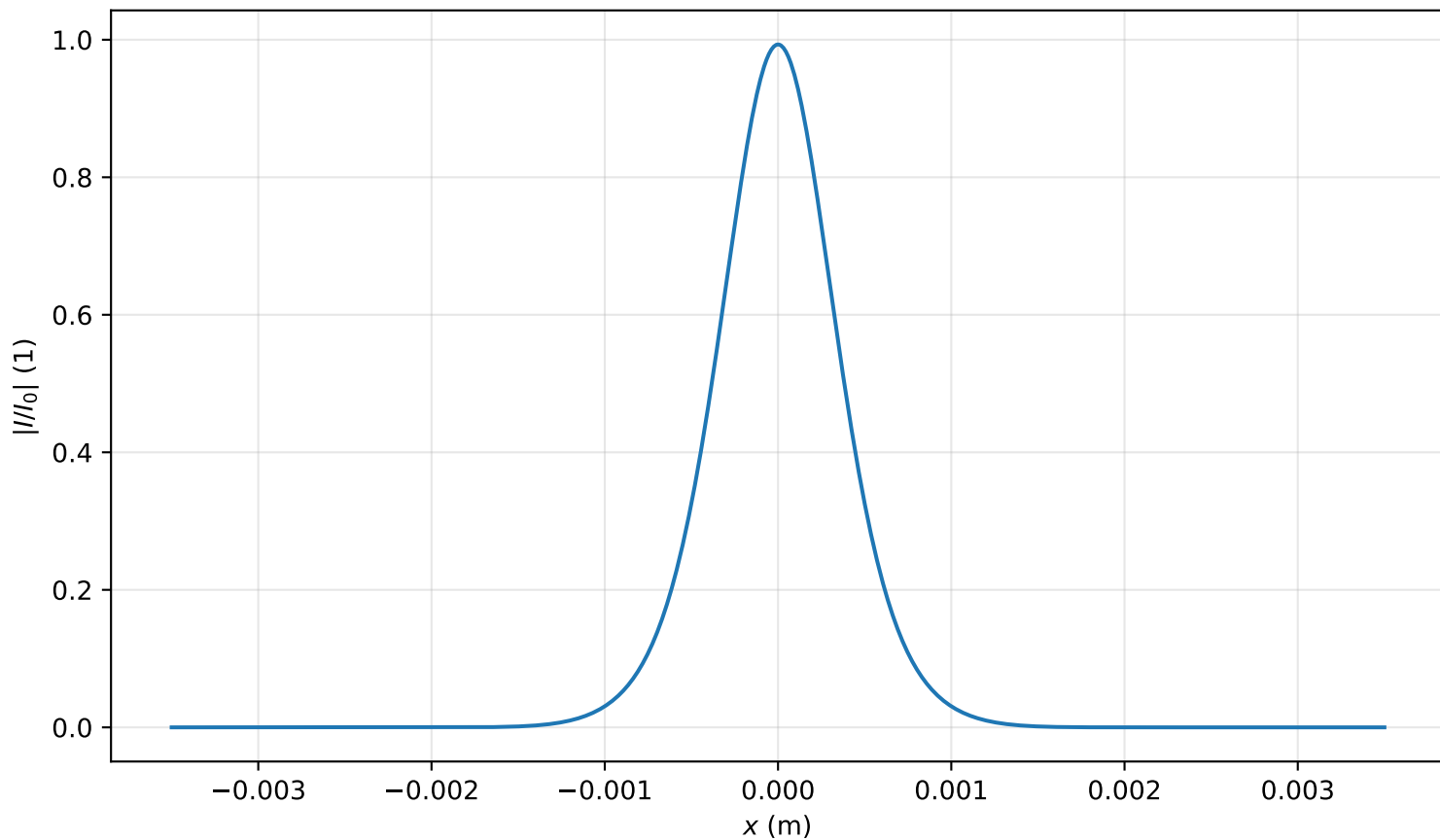
Intensity profile I(x, y = 0, z = 1.353m)/I_0 , P_{in}=0.5P_{cr} , artificial time
